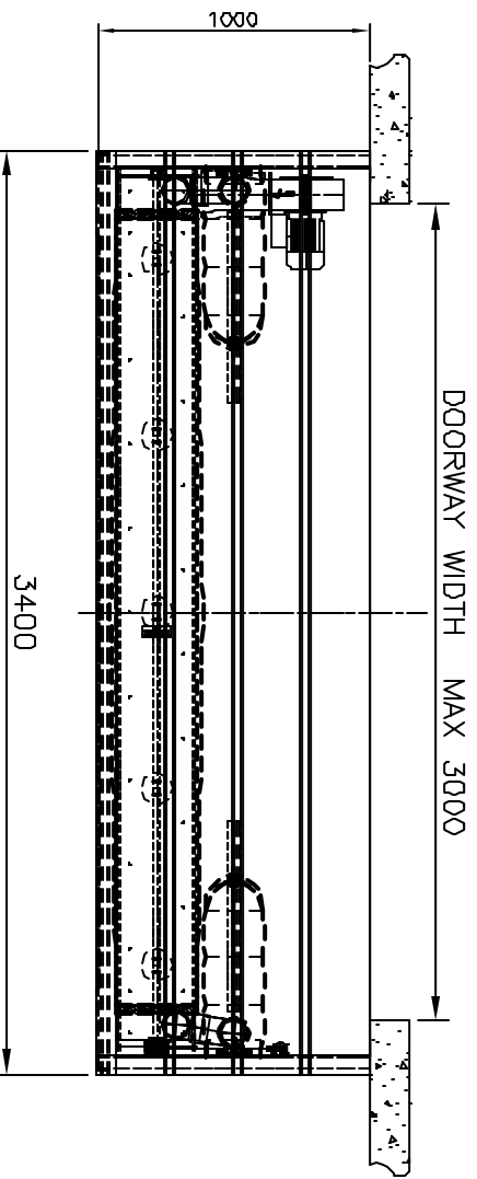
PLAN
