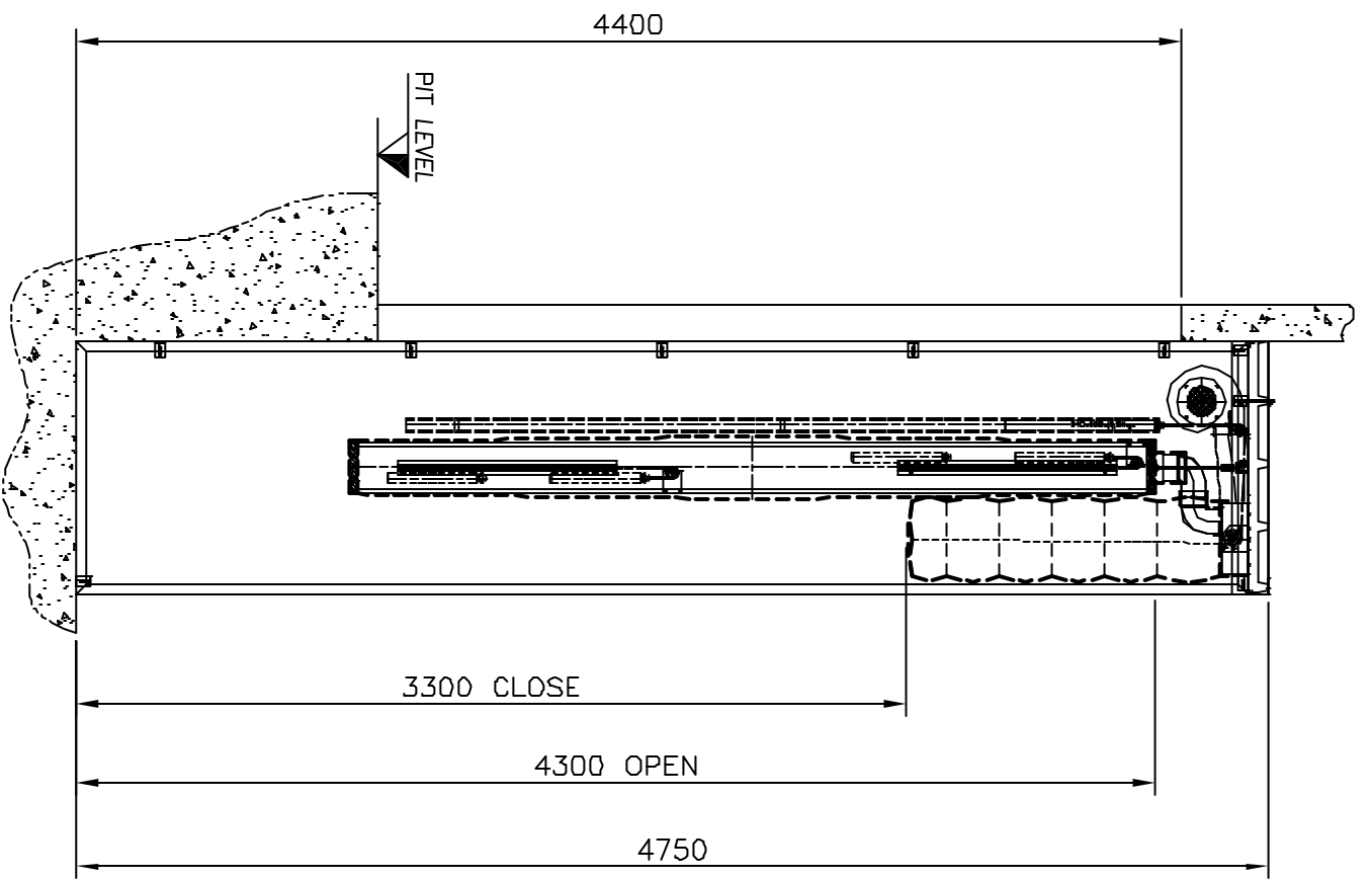
SIDE VIEW
