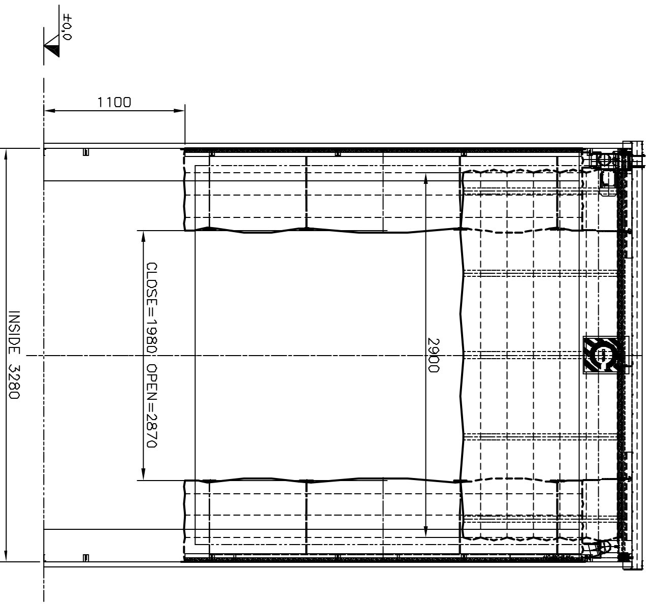
FRONT VIEW
