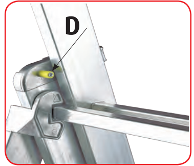
Device to prevent third section overturning (LUXE 3).
